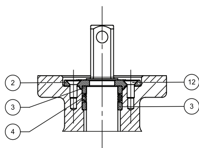
SECTION C-C SCALE 1: 1
